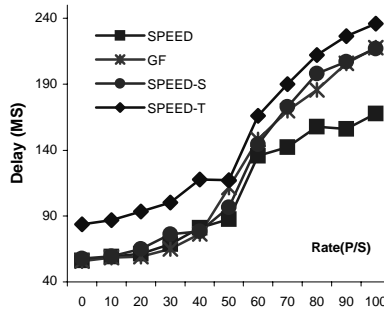
Figure 8. E2E Delay Under Different Congestion
